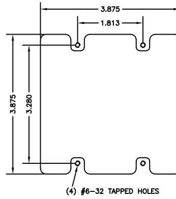
DOUBLE GANG MOUNT
