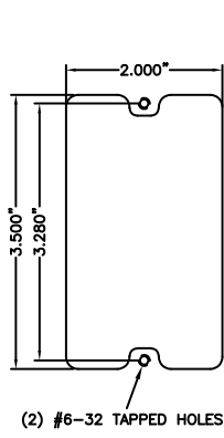
SINGLE GANG MOUNT
