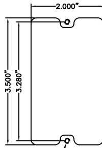
SINGLE GANG MOUNT
