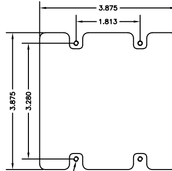
DOUBLE GANG MOUNT
